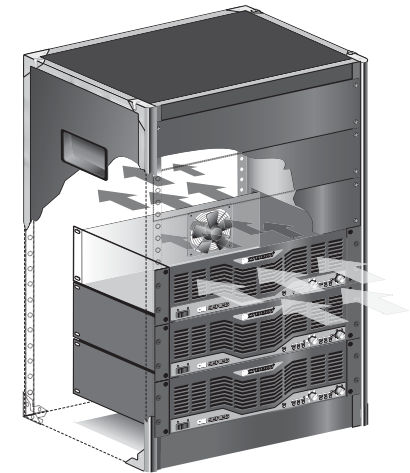
Figure 3.2 Airflow
