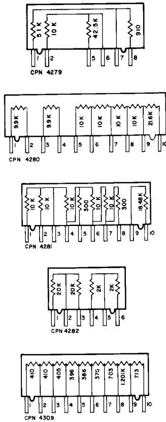
Fig. 4.2 Resistor Networks.
