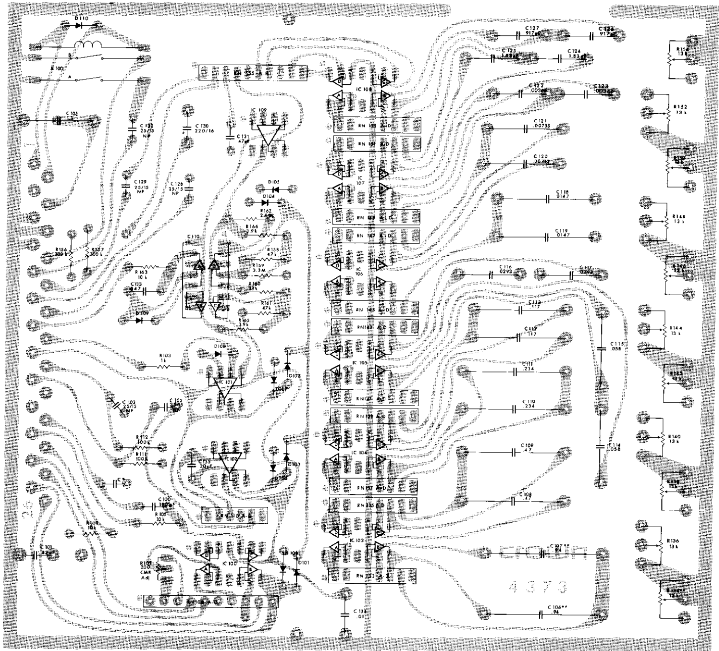
Fig. 6.4 Main PC Board
