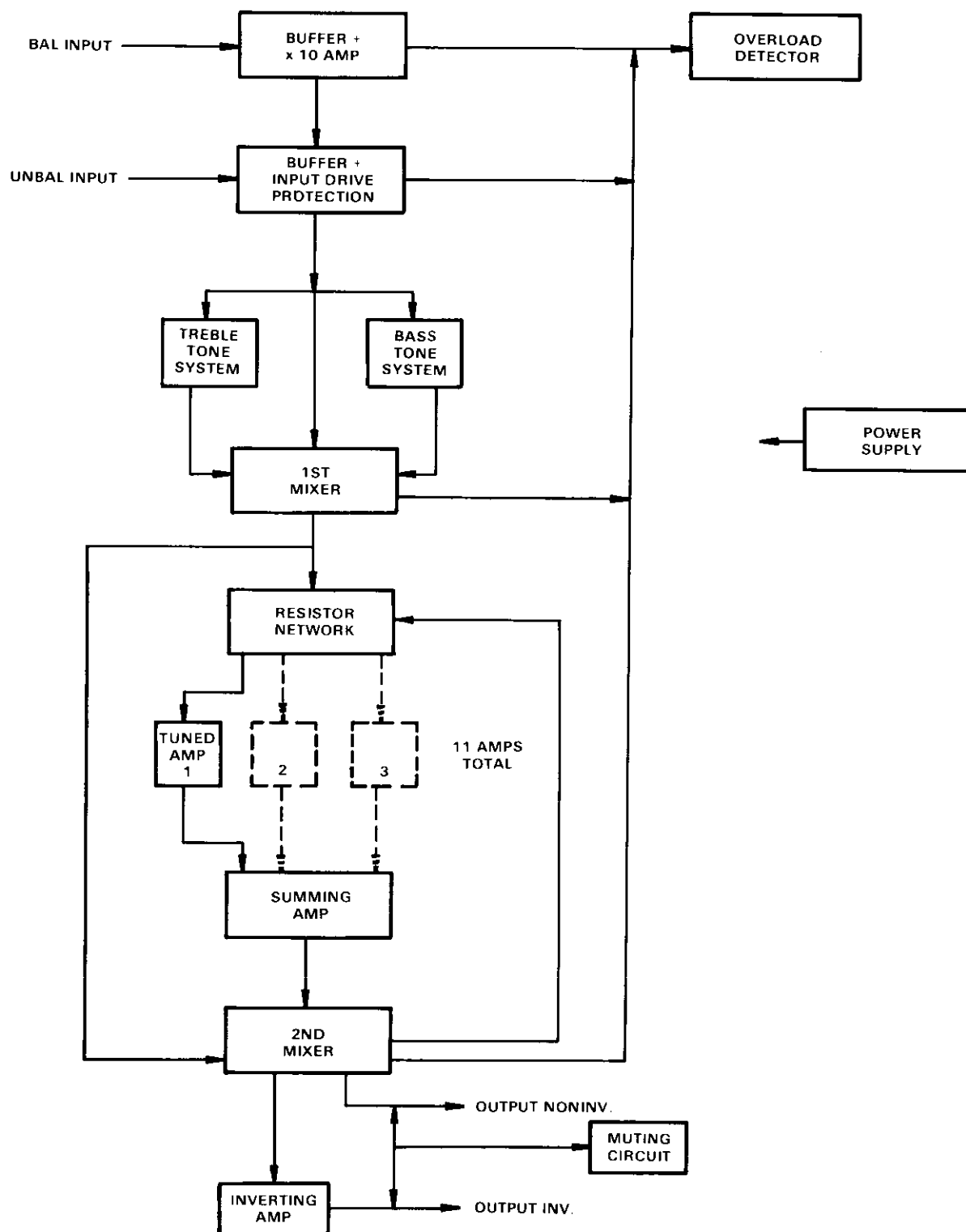
Fig. 4.1 Block Diagram.
