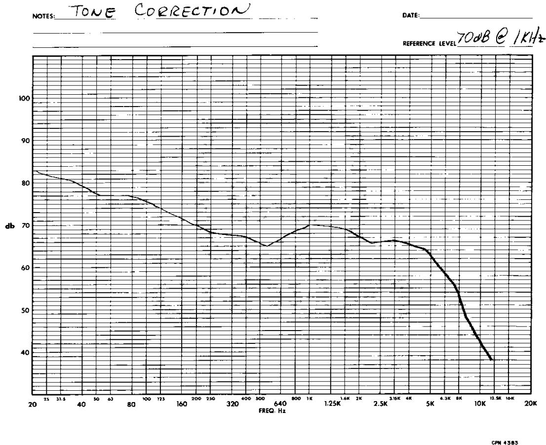
Fig. 3.19 Typical Graph After Tone Correction.
