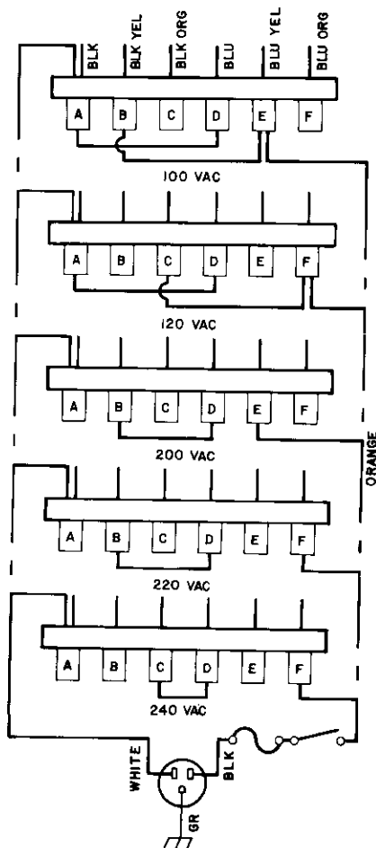
Fig. 3.4 Modifying AC Mains Voltage.
