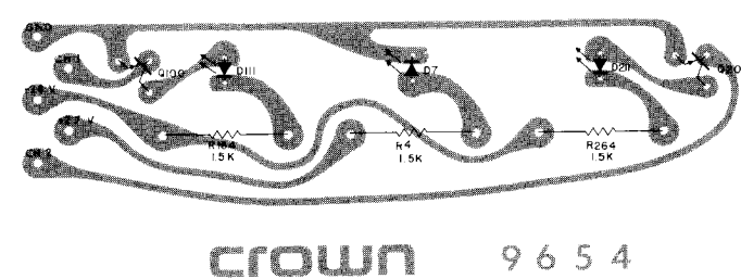
Fig. 4.5 Display P.C. Board.
