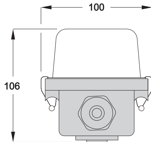
Cyclo IP65 02 and 28 W tube Cyclo IP65 03
