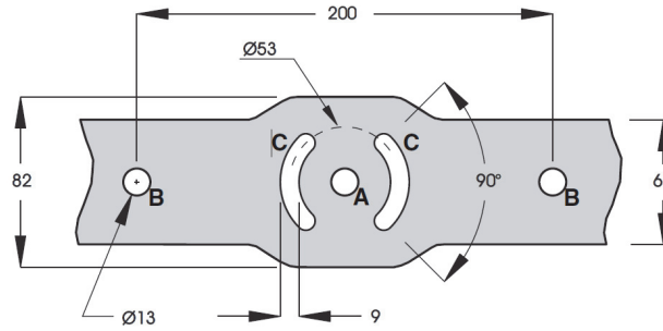
Mounting bracket details
