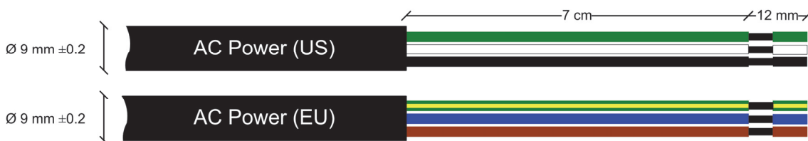
AC power cable details
