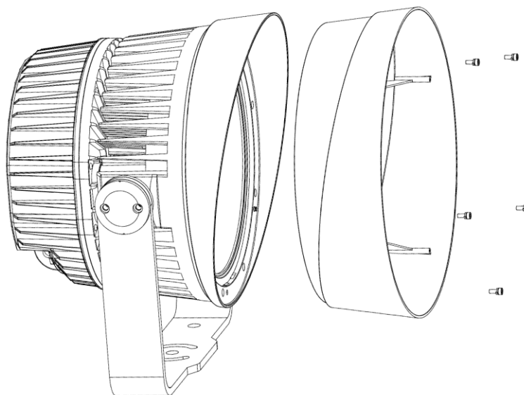
Snoot installation
