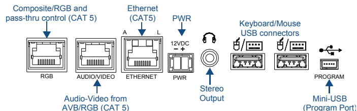
FIG. 2 Connector layout
