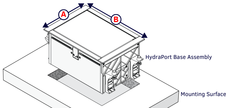
FIG. 1 ABOVE-SURFACE DIMENSIONS OF HPX BASE ASSEMBLIES
