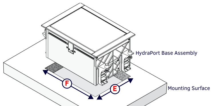
FIG. 4 HOLE CUTOUT DIMENSIONS FOR THE MOUNTING SURFACE
