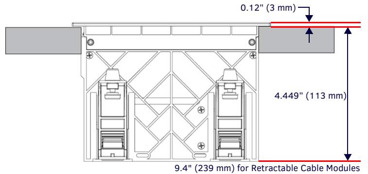
FIG. 2 DIMENSIONS OF THE HPX BASE ASSEMBLY (BELOW THE TABLE)
