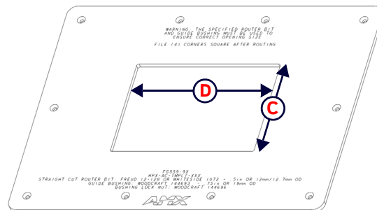
FIG. 3 HPX-AC-TMPLT ROUTER GUIDES - ROUTING AREA
