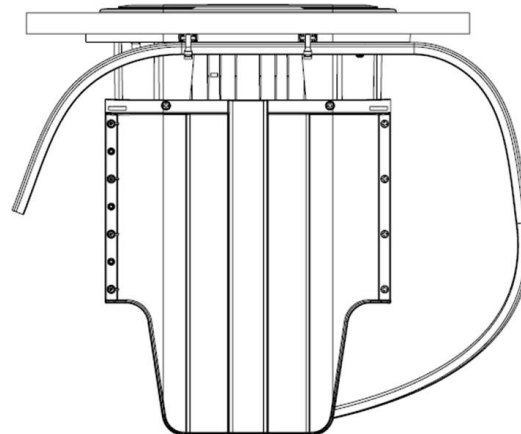
FIG. 5 SECURED SERVICE LOOP
