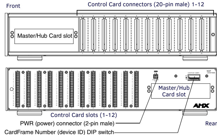
FIG. 2 NXF CARDFRAME - FRONT/REAR PANEL COMPONENTS
