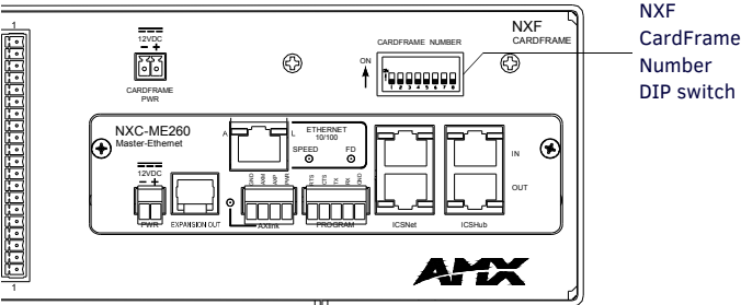
FIG. 3 CARDFRAME NUMBER DIP SWITCH (8-POSITION)
