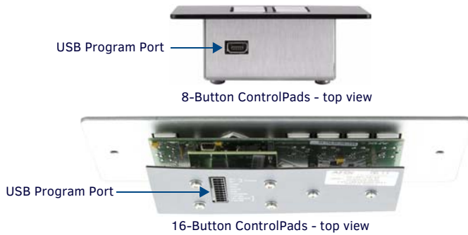
FIG. 3 USB PROGRAM PORT
