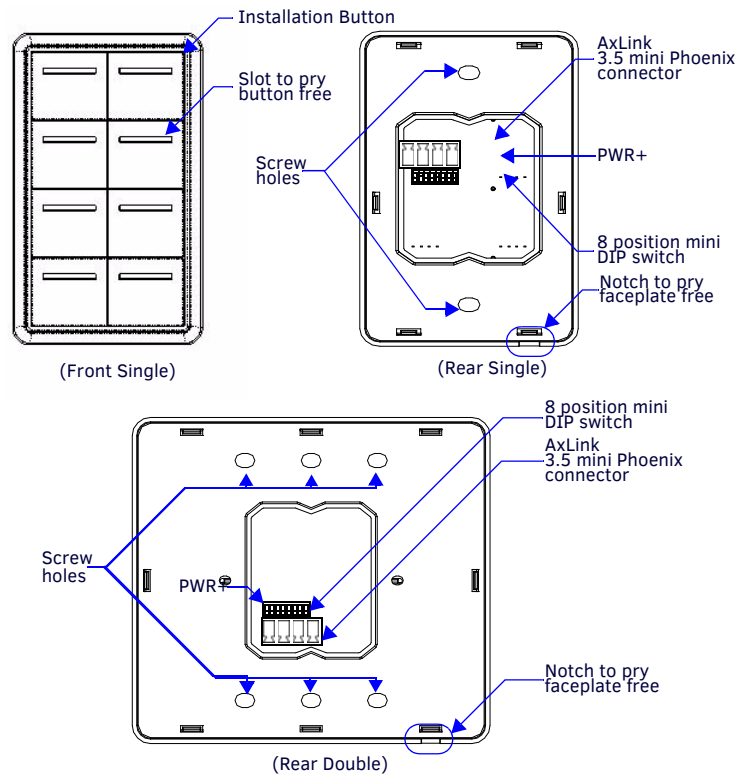
FIG. 2 MIO MODERO FRONT AND REAR COMPONENTS
