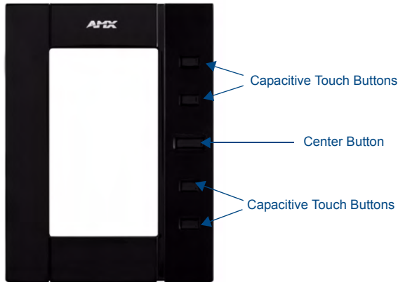
FIG. 1 NXA-435-BL 4.3" Portrait Bezel for the NXD-435 Touch Panel
