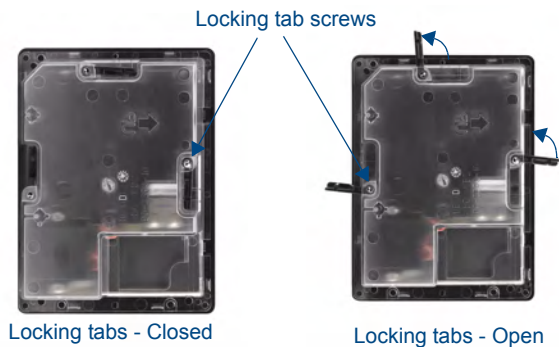
FIG. 3 NXD-435 backbox with closed and open locking tabs
