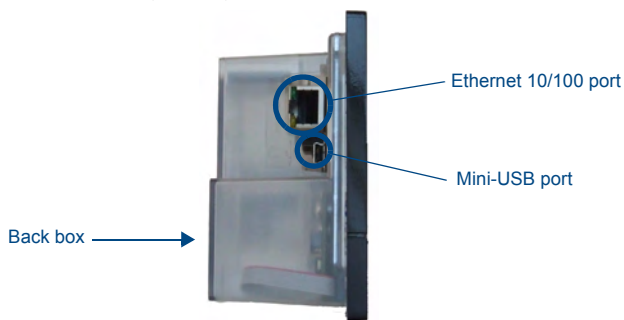
FIG. 2 Connector layout on the NXD-435 Modero Wall/Flush Touch Panel
