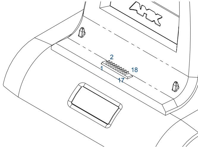
FIG. 16 MVP-TDS Connector Pin locations and Pinout function
