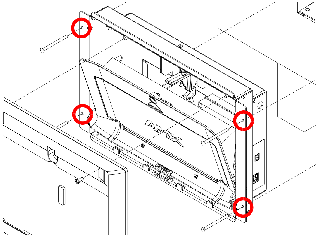
FIG. 10 Installing four #6-32 Mounting Screws in Step 3
