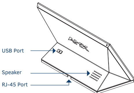
FIG. 2 MT-1002 (REAR VIEW)
