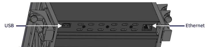
FIG. 8 HPX BOTTOM VIEW - ETHERNET AND USB PORTS
