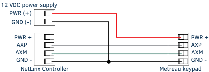
FIG. 5 AXLINK AND 12 VDC POWER SUPPLY WIRING DIAGRAM
