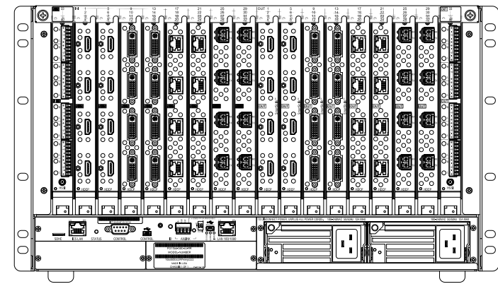
BACK VIEW (SAMPLE CONFIGURATION)
