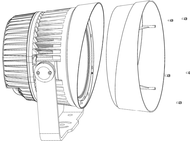
Snoot installation
