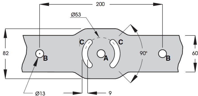
Mounting bracket details
