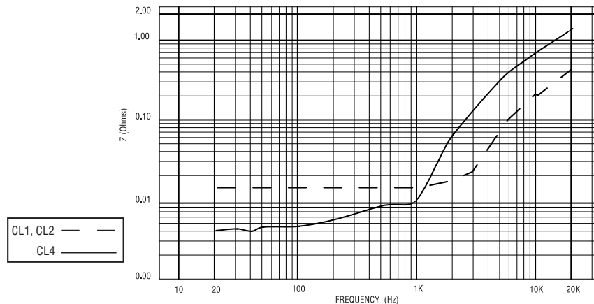
Figure 1 CL1, CL2, CL4 Output Impedance
